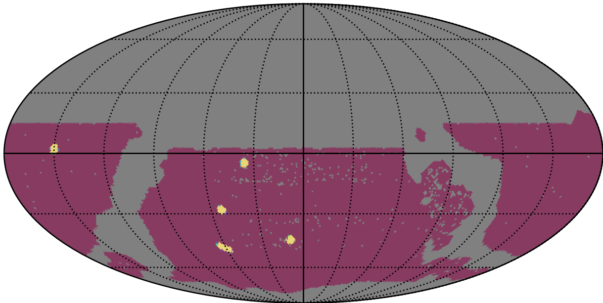
too_elab_r16_d2_giz_v3.4_10yrs WFD: NumberOfQuickRevisits
