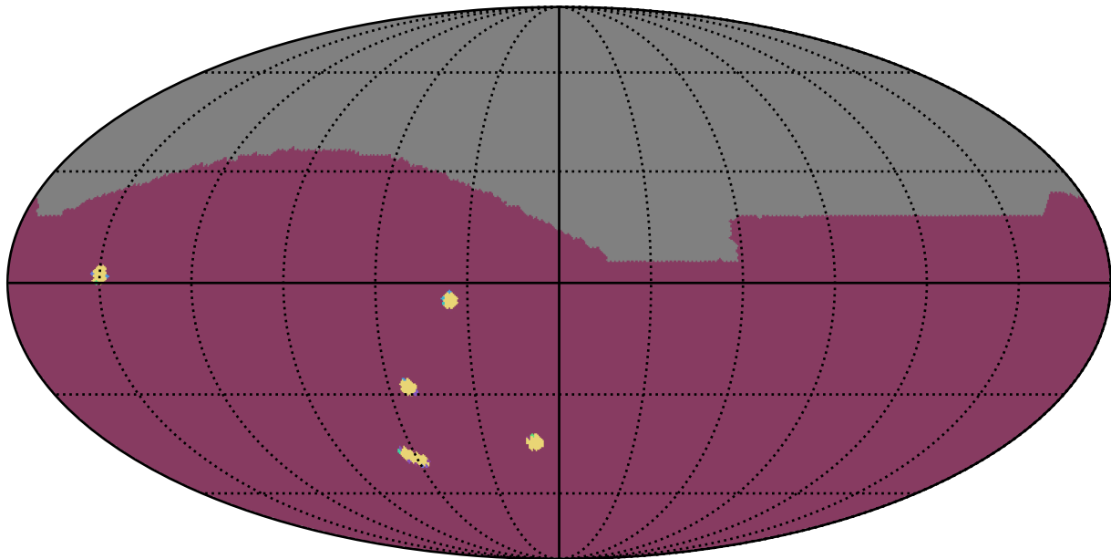
too_elab_r16_d2_giz_v3.4_10yrs All sky: NumberOfQuickRevisits
