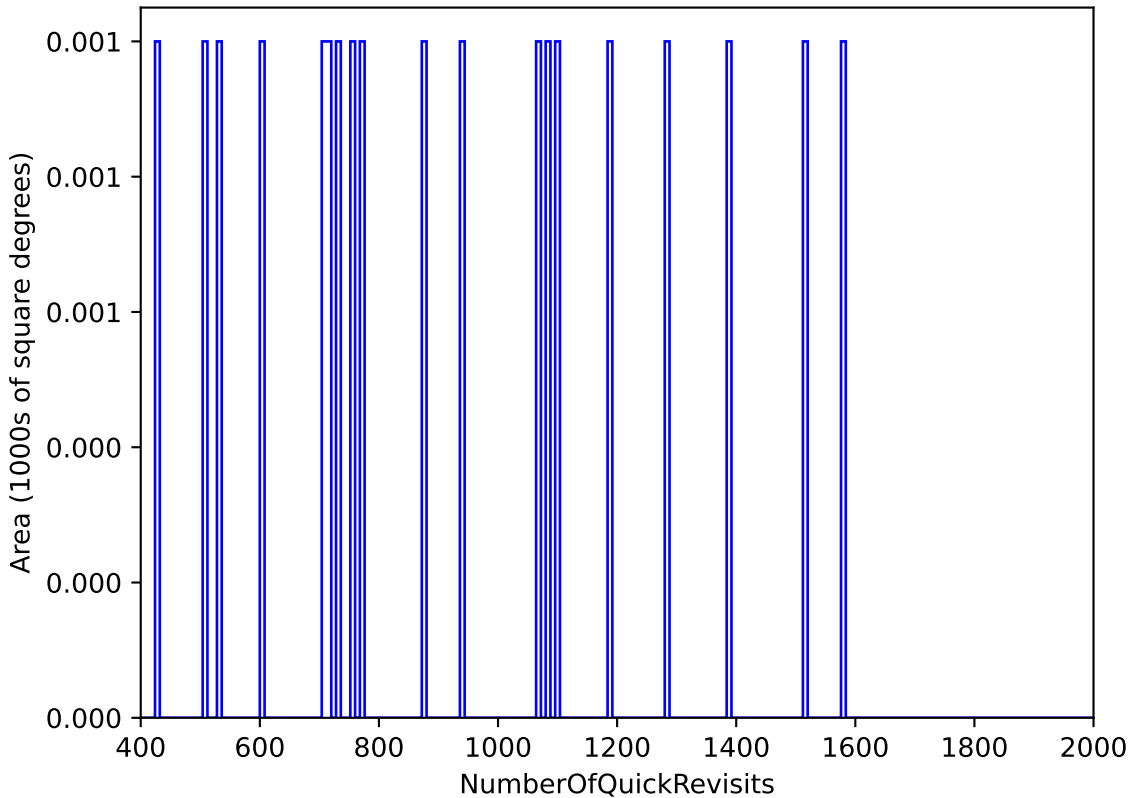
too_elab_r16_d2_giz_v3.4_10yrs All sky: NumberOfQuickRevisits
