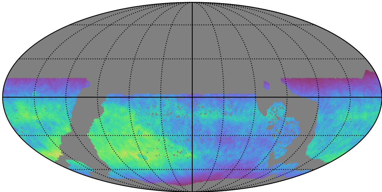
too_elab_r16_d2_giz_v3.4_10yrs WFD z band: Normalized Teff
