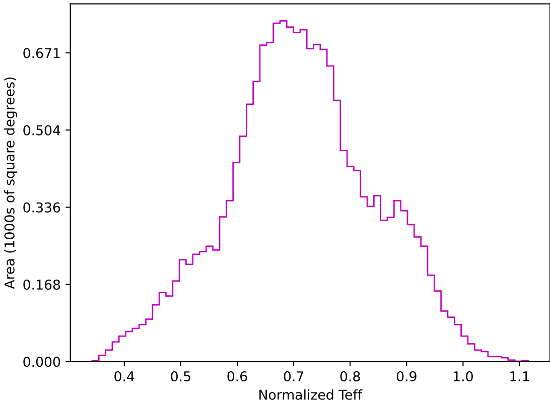
too_elab_r16_d2_giz_v3.4_10yrs WFD z band: Normalized Teff
