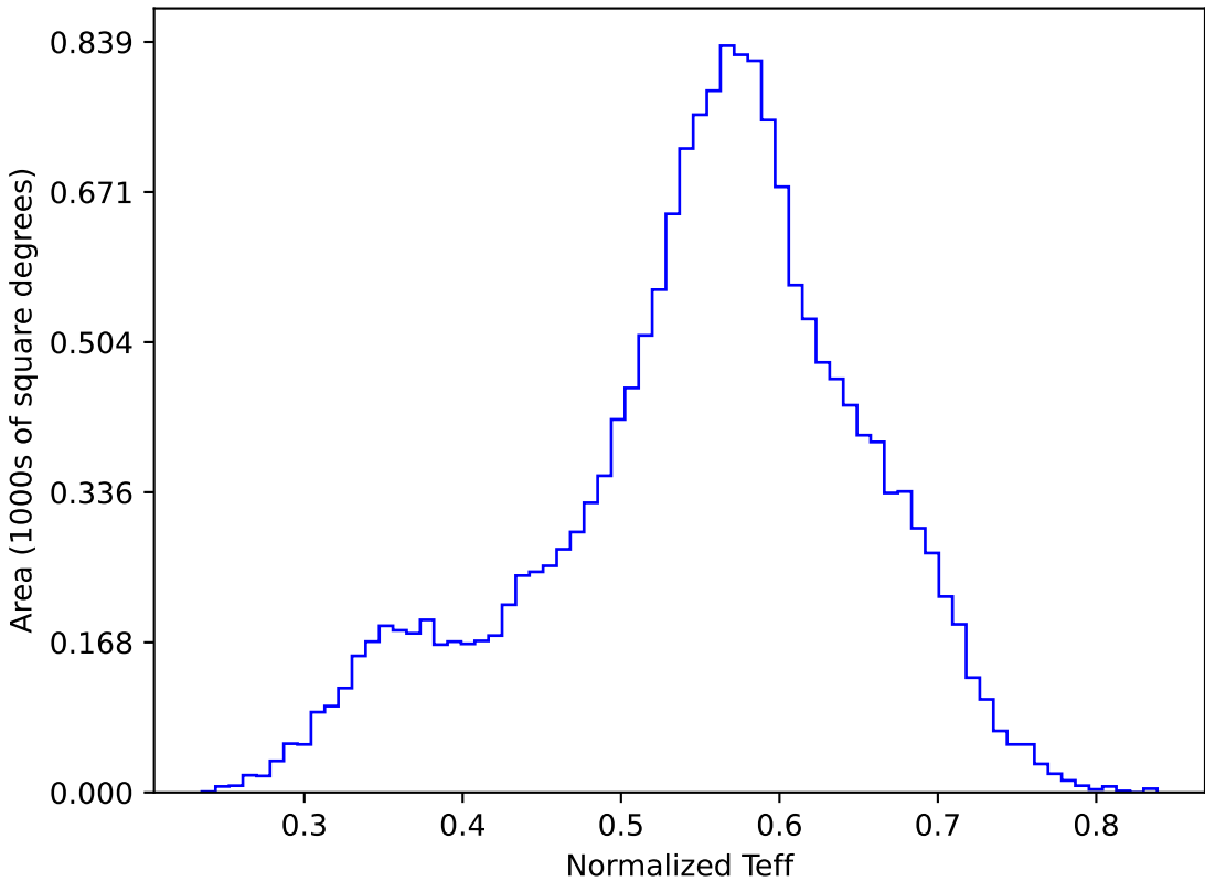
too_elab_r16_d2_giz_v3.4_10yrs WFD y band: Normalized Teff
