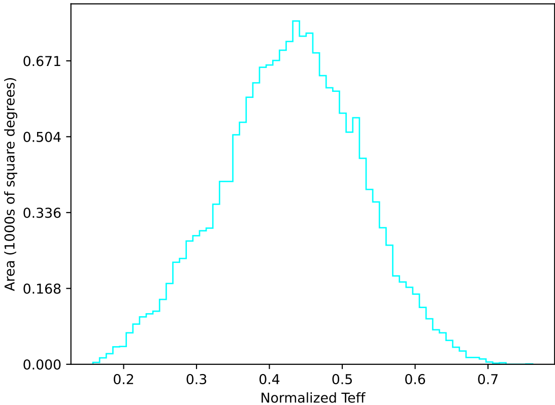
too_elab_r16_d2_giz_v3.4_10yrs WFD u band: Normalized Teff
