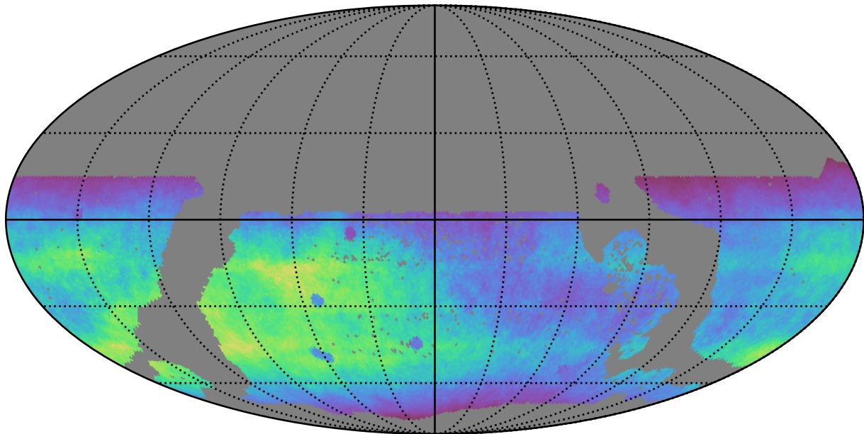
too_elab_r16_d2_giz_v3.4_10yrs WFD r band: Normalized Teff
