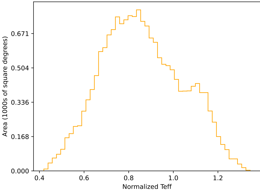
too_elab_r16_d2_giz_v3.4_10yrs WFD r band: Normalized Teff
