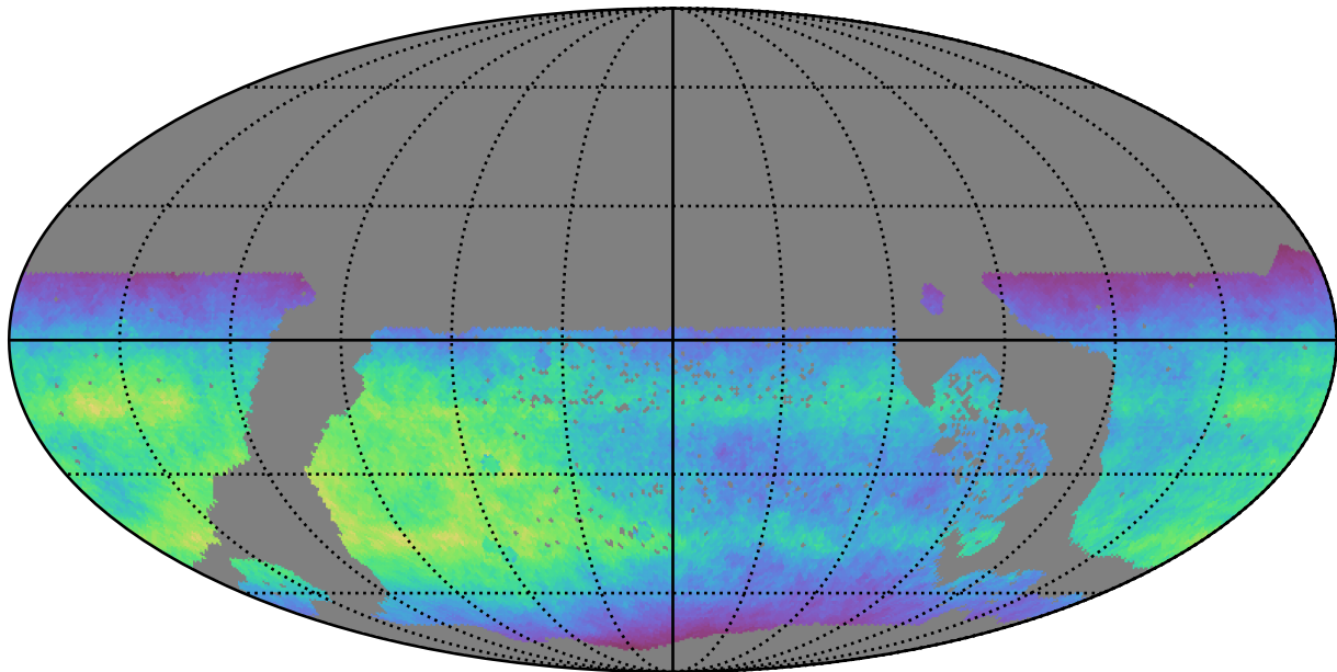
too_elab_r16_d2_giz_v3.4_10yrs WFD i band: Normalized Teff
