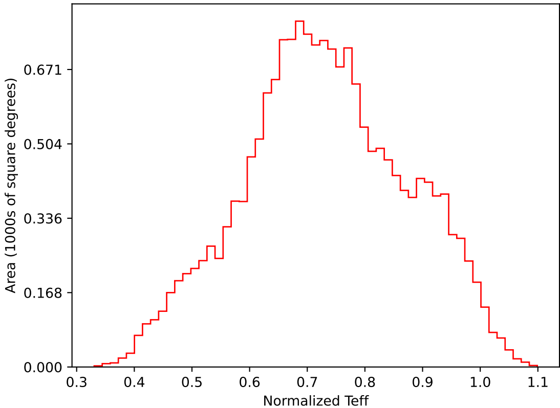
too_elab_r16_d2_giz_v3.4_10yrs WFD i band: Normalized Teff
