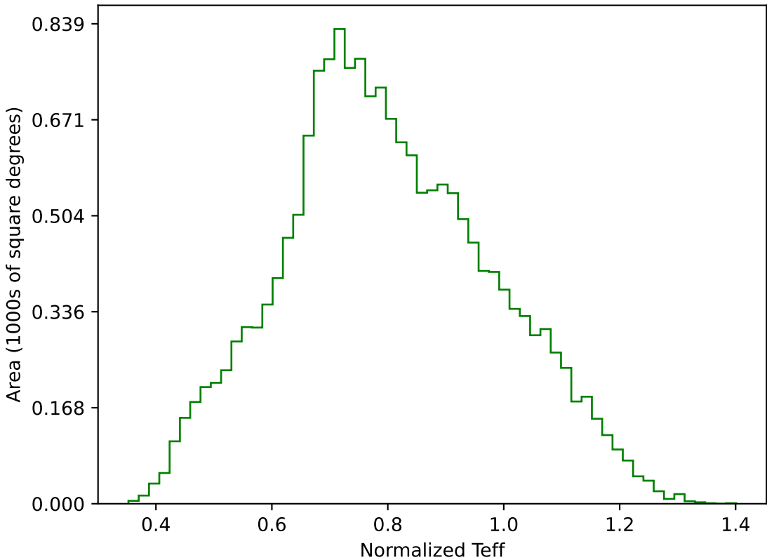
too_elab_r16_d2_giz_v3.4_10yrs WFD g band: Normalized Teff
