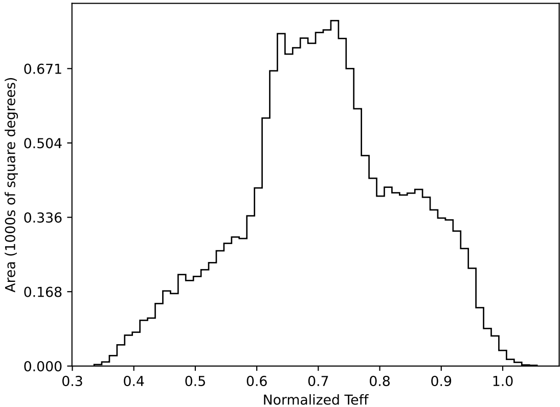
too_elab_r16_d2_giz_v3.4_10yrs WFD all bands: Normalized Teff
