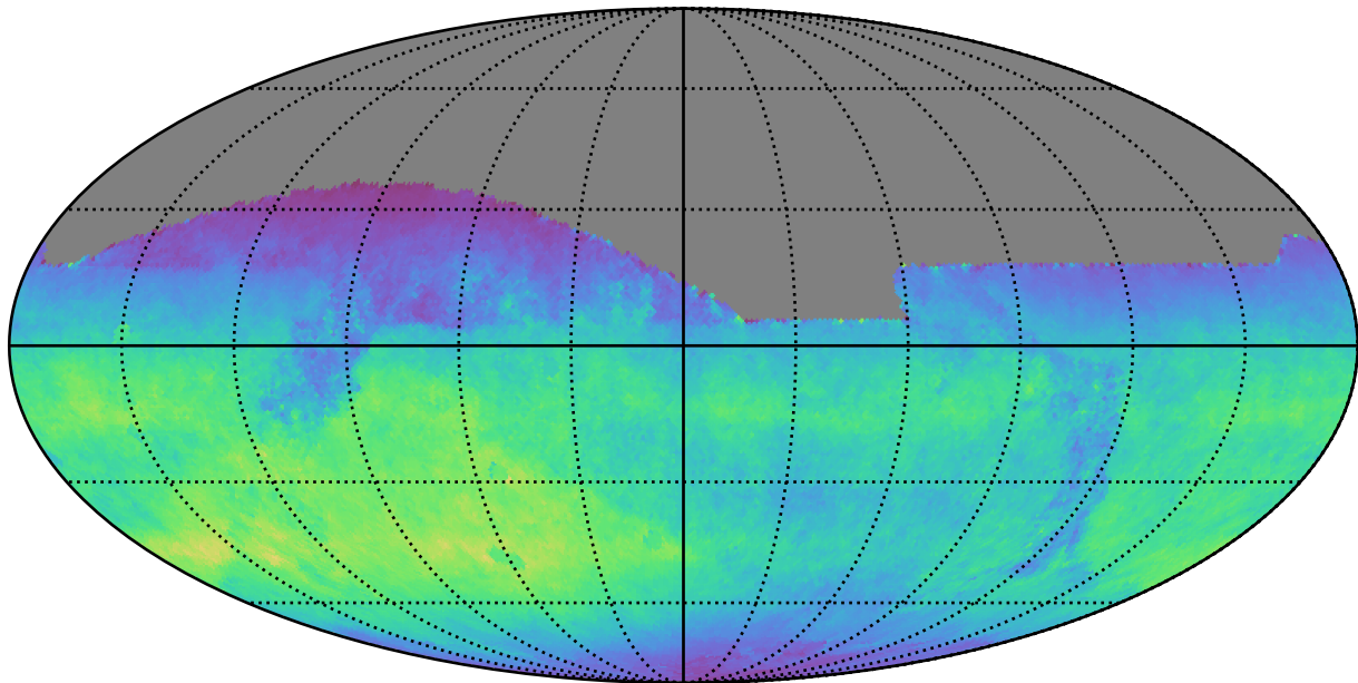
too_elab_r16_d2_giz_v3.4_10yrs All sky z band: Normalized Teff
