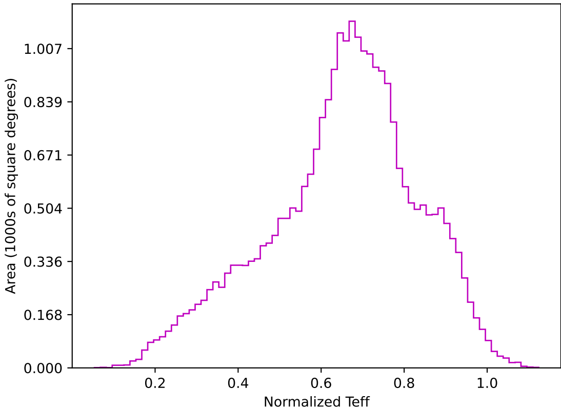
too_elab_r16_d2_giz_v3.4_10yrs All sky z band: Normalized Teff
