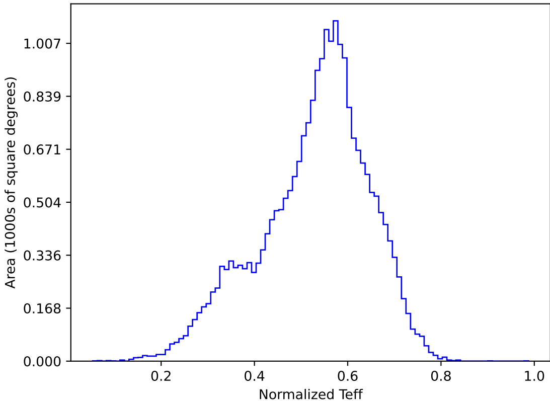
too_elab_r16_d2_giz_v3.4_10yrs All sky y band: Normalized Teff
