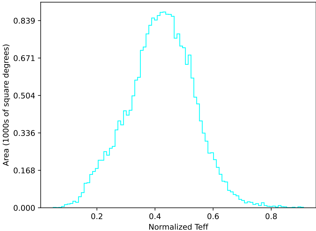
too_elab_r16_d2_giz_v3.4_10yrs All sky u band: Normalized Teff
