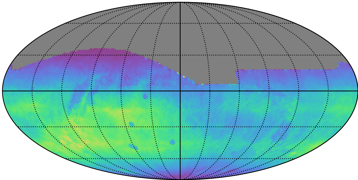
too_elab_r16_d2_giz_v3.4_10yrs All sky r band: Normalized Teff
