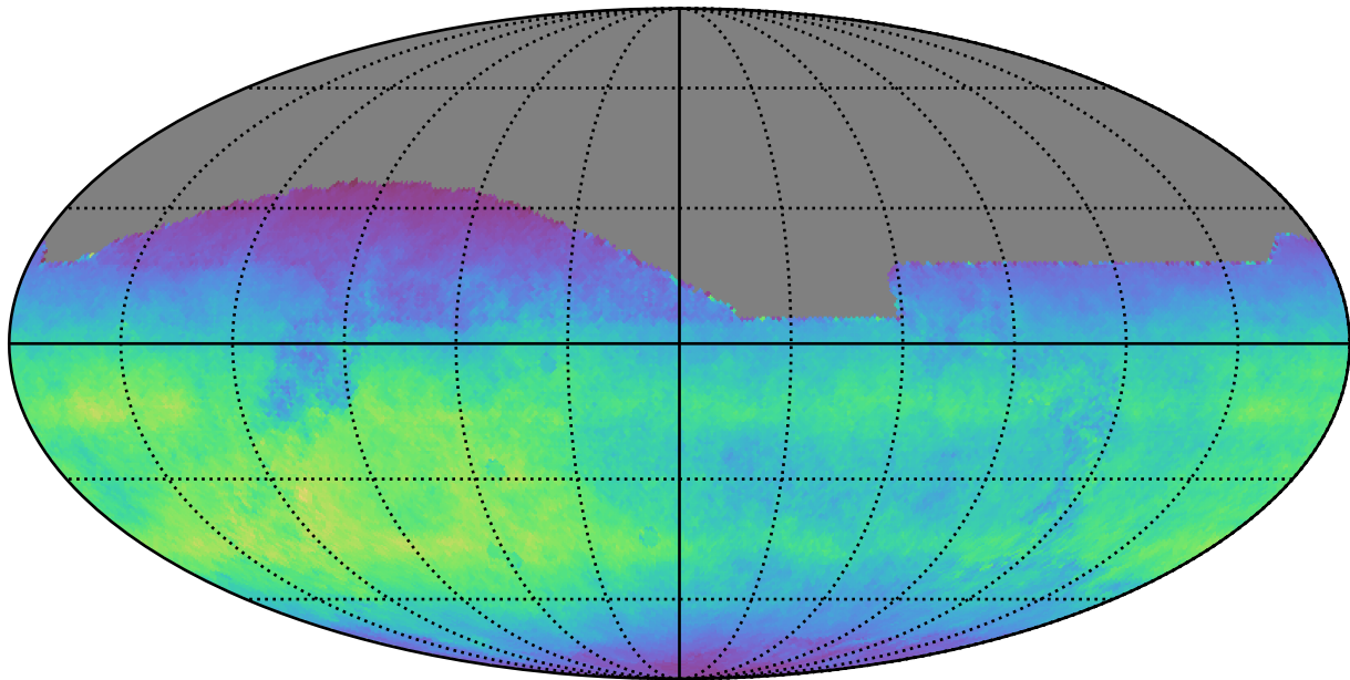
too_elab_r16_d2_giz_v3.4_10yrs All sky i band: Normalized Teff
