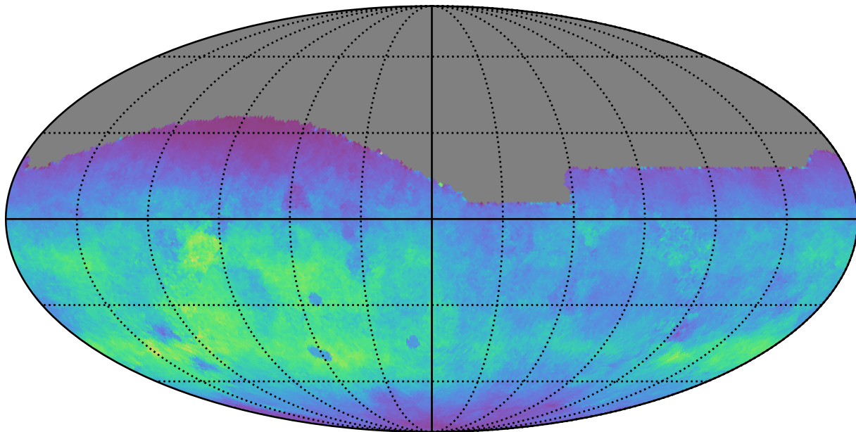
too_elab_r16_d2_giz_v3.4_10yrs All sky g band: Normalized Teff
