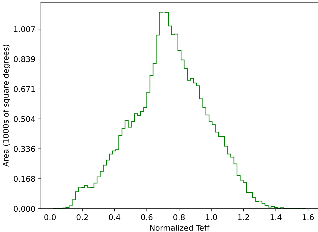
too_elab_r16_d2_giz_v3.4_10yrs All sky g band: Normalized Teff
