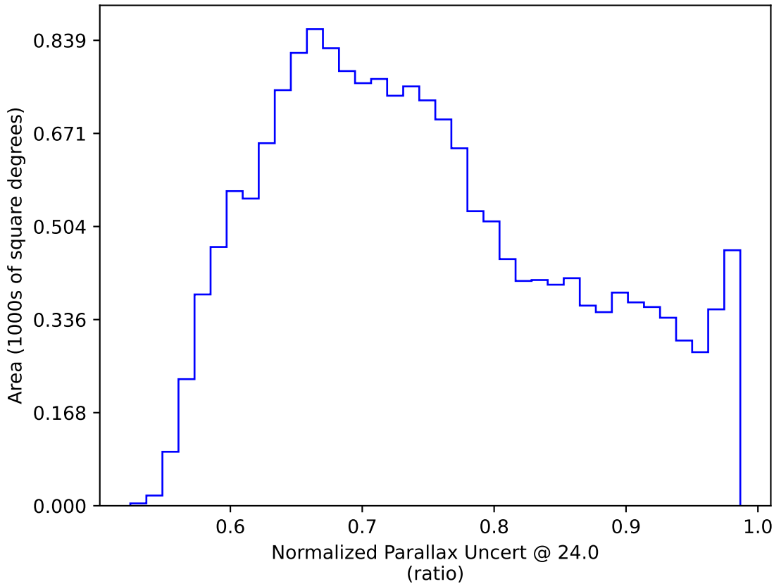
too_elab_r16_d2_giz_v3.4_10yrs WFD: Normalized Parallax Uncert @ 24.0
