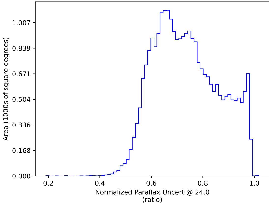
too_elab_r16_d2_giz_v3.4_10yrs All sky: Normalized Parallax Uncert @ 24.0
