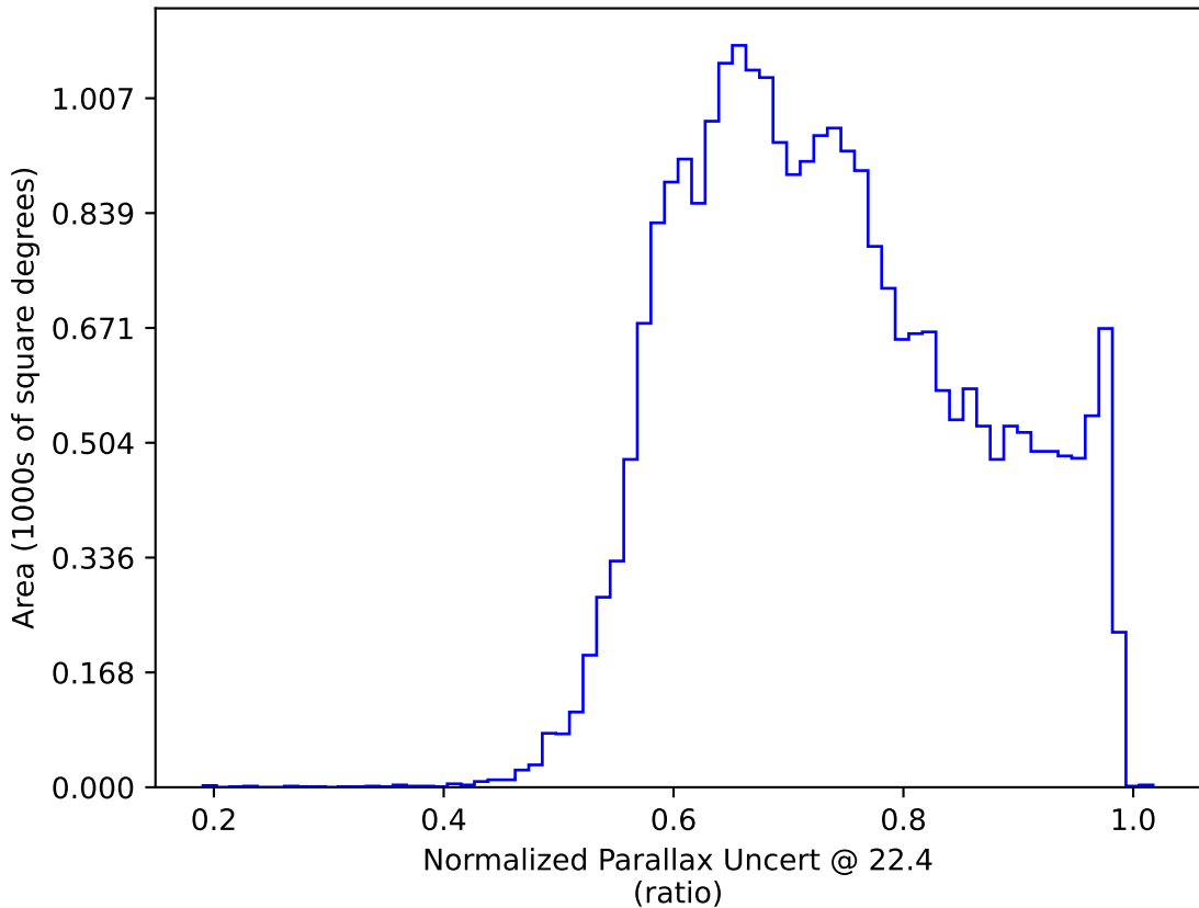
too_elab_r16_d2_giz_v3.4_10yrs All sky: Normalized Parallax Uncert @ 22.4
