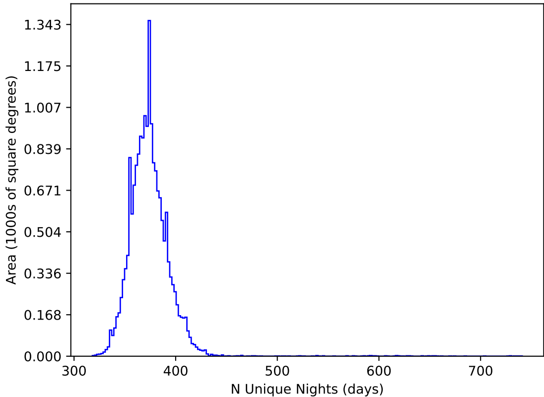
too_elab_r16_d2_giz_v3.4_10yrs WFD all bands: N Unique Nights
