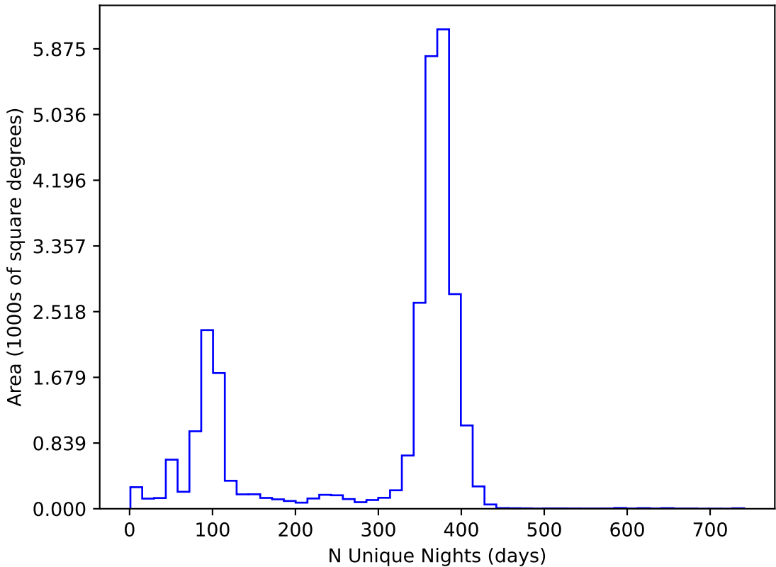
too_elab_r16_d2_giz_v3.4_10yrs All sky all bands: N Unique Nights
