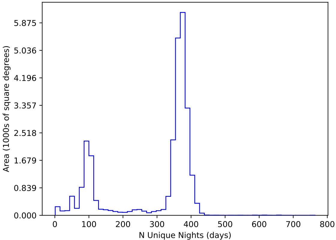
too_elab_r16_d2_giz_v3.4_10yrs All sky all bands: N Unique Nights
