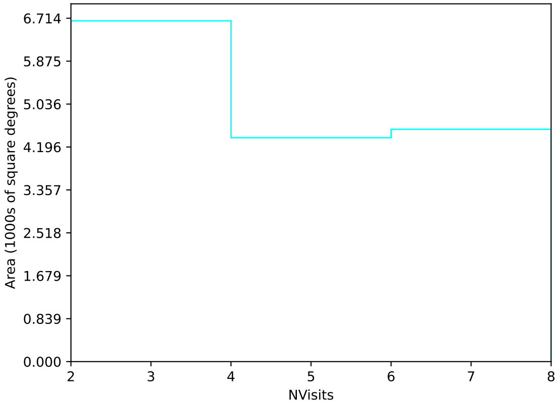
too_elab_r16_d2_giz_v3.4_10yrs Yr 3-4 u band: NVisits
