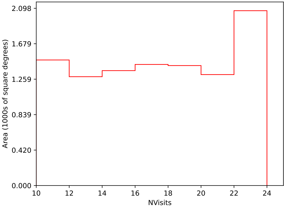
too_elab_r16_d2_giz_v3.4_10yrs Yr 3-4 i band: NVisits
