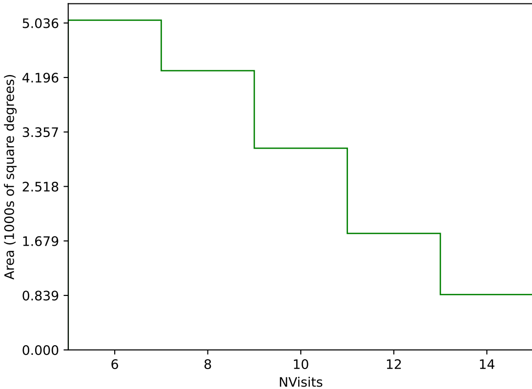
too_elab_r16_d2_giz_v3.4_10yrs Yr 3-4 g band: NVisits
