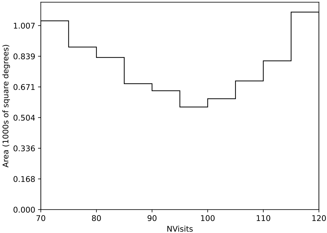
too_elab_r16_d2_giz_v3.4_10yrs Yr 3-4 all bands: NVisits
