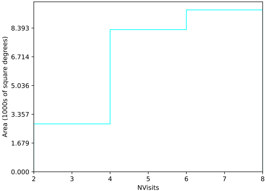
too_elab_r16_d2_giz_v3.4_10yrs Yr 1 u band: NVisits
