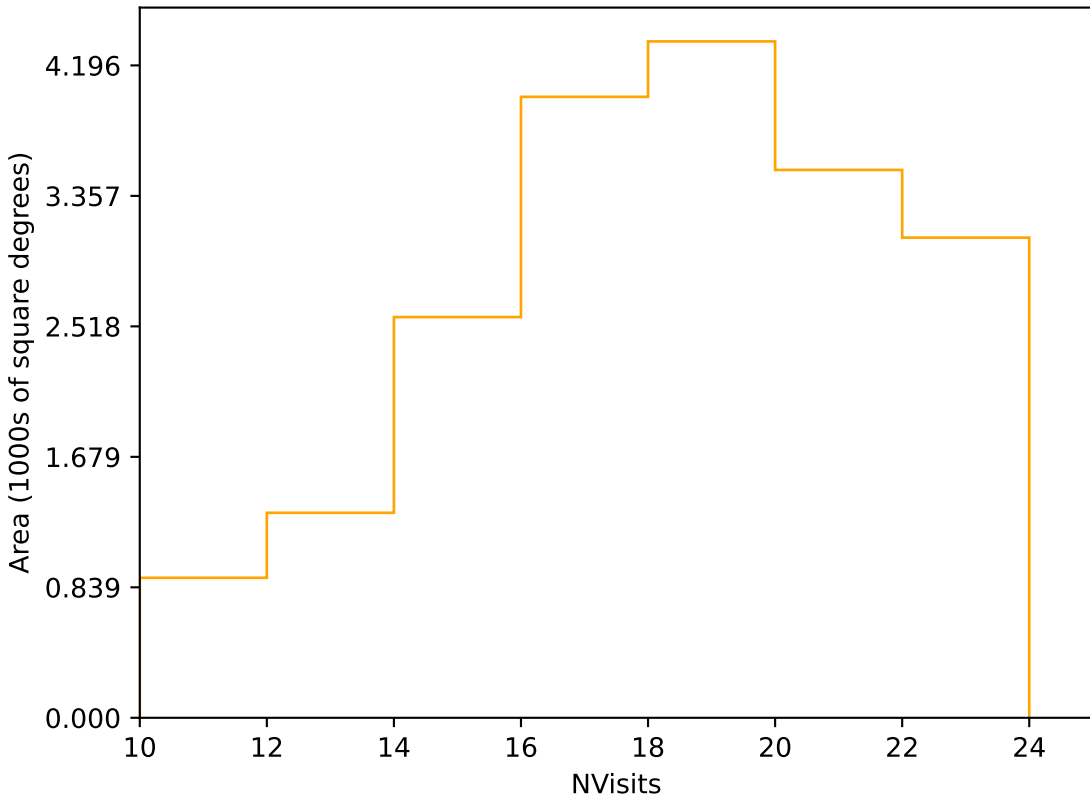
too_elab_r16_d2_giz_v3.4_10yrs Yr 1 r band: NVisits
