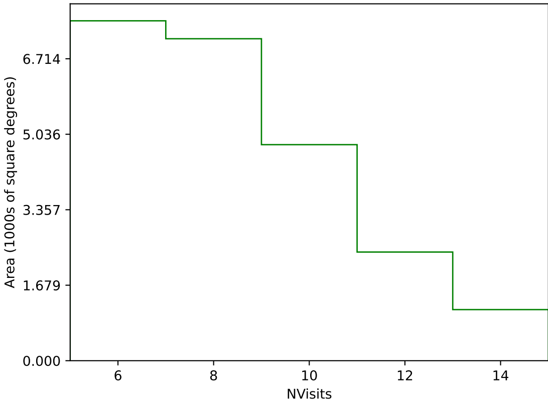
too_elab_r16_d2_giz_v3.4_10yrs Yr 1 g band: NVisits
