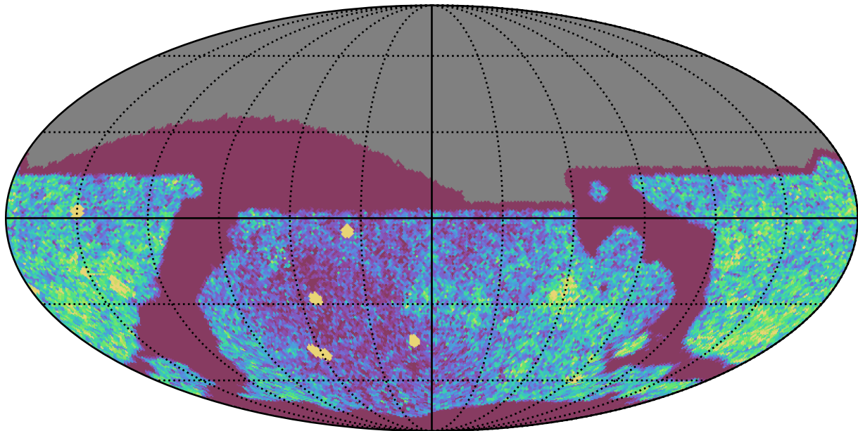
too_elab_r16_d2_giz_v3.4_10yrs Yr 1 all bands: NVisits
