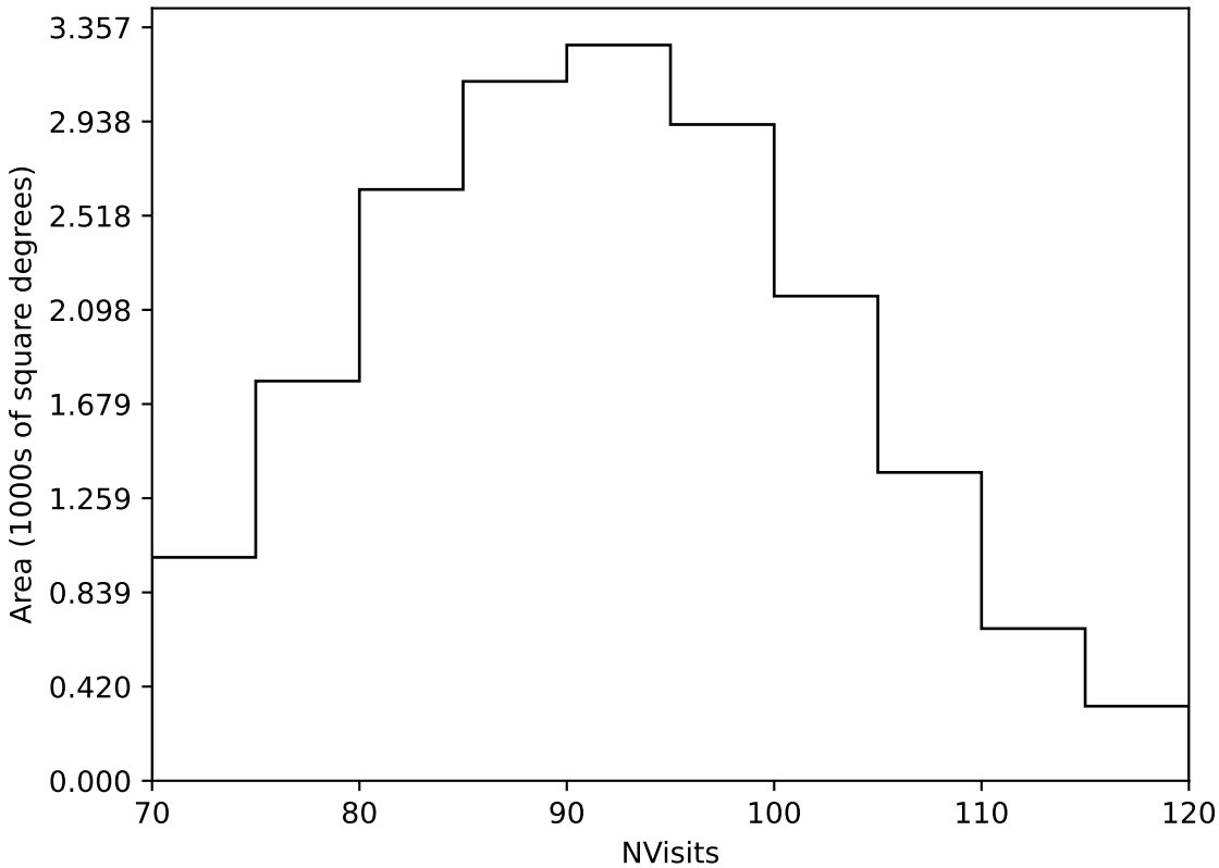
too_elab_r16_d2_giz_v3.4_10yrs Yr 1 all bands: NVisits
