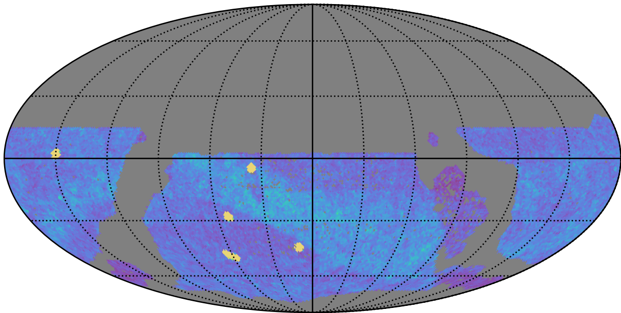
too_elab_r16_d2_giz_v3.4_10yrs WFD z band: NVisits
