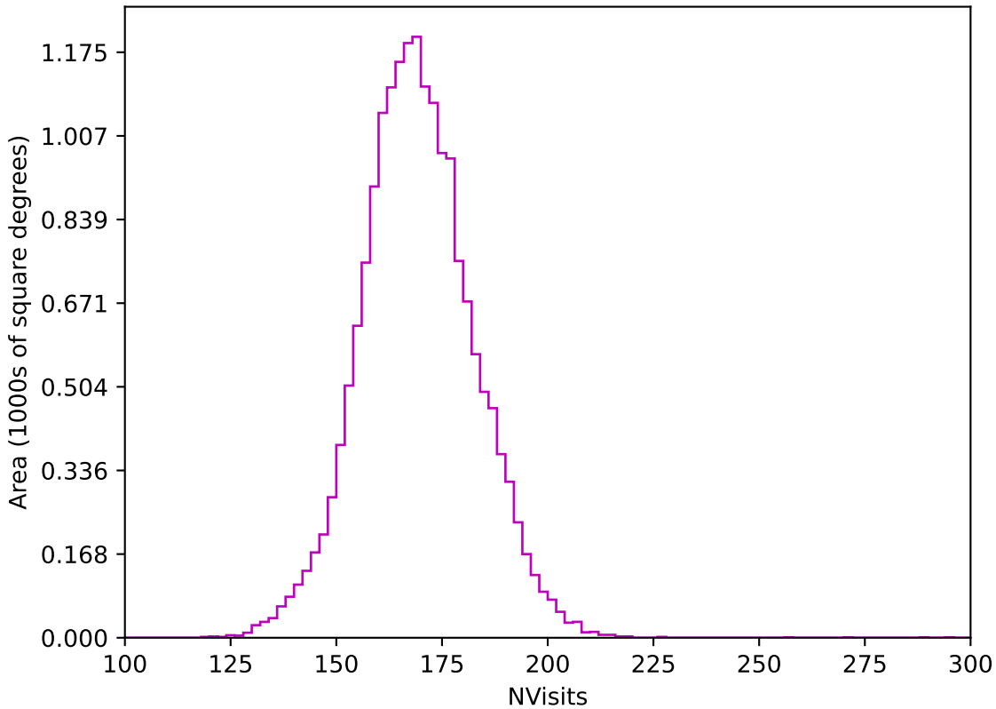
too_elab_r16_d2_giz_v3.4_10yrs WFD z band: NVisits
