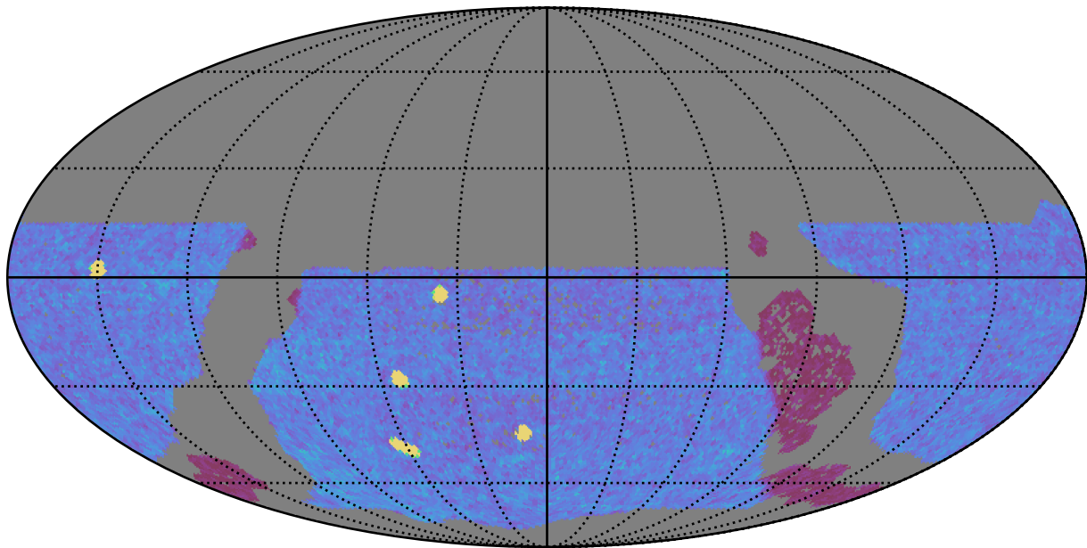
too_elab_r16_d2_giz_v3.4_10yrs WFD y band: NVisits
