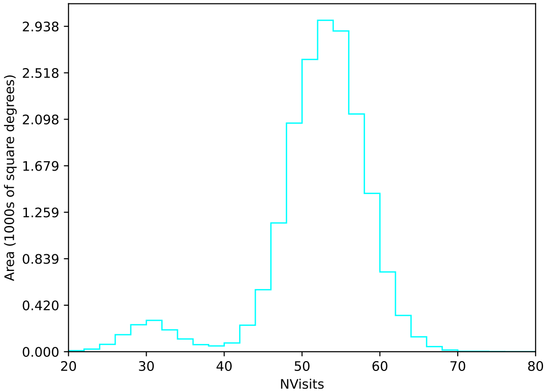
too_elab_r16_d2_giz_v3.4_10yrs WFD u band: NVisits
