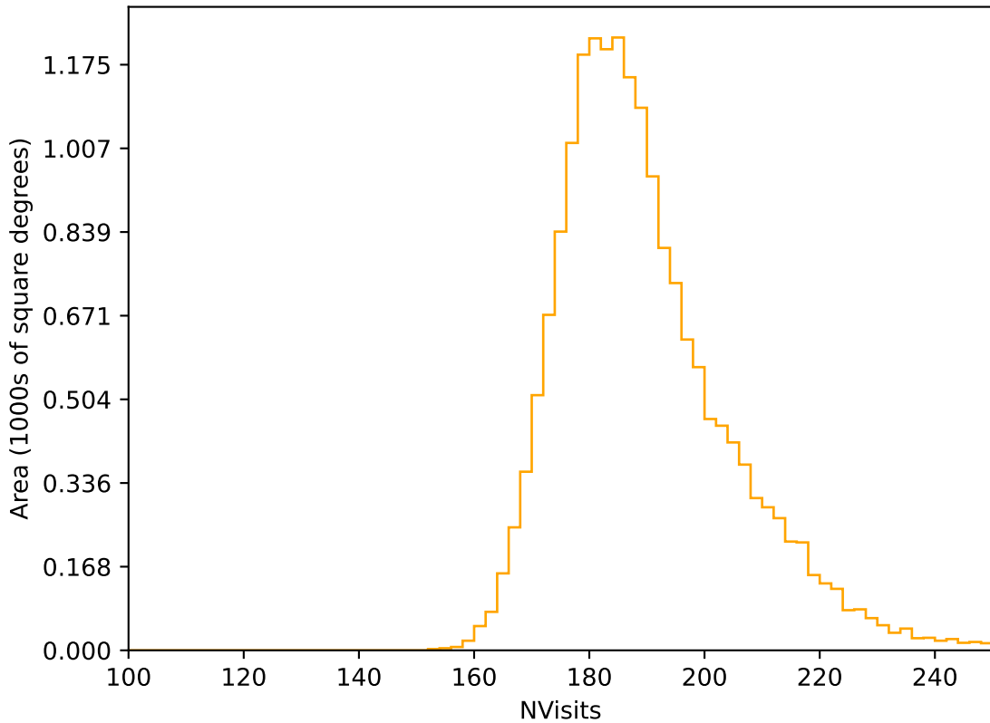
too_elab_r16_d2_giz_v3.4_10yrs WFD r band: NVisits
