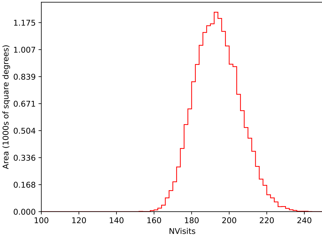
too_elab_r16_d2_giz_v3.4_10yrs WFD i band: NVisits
