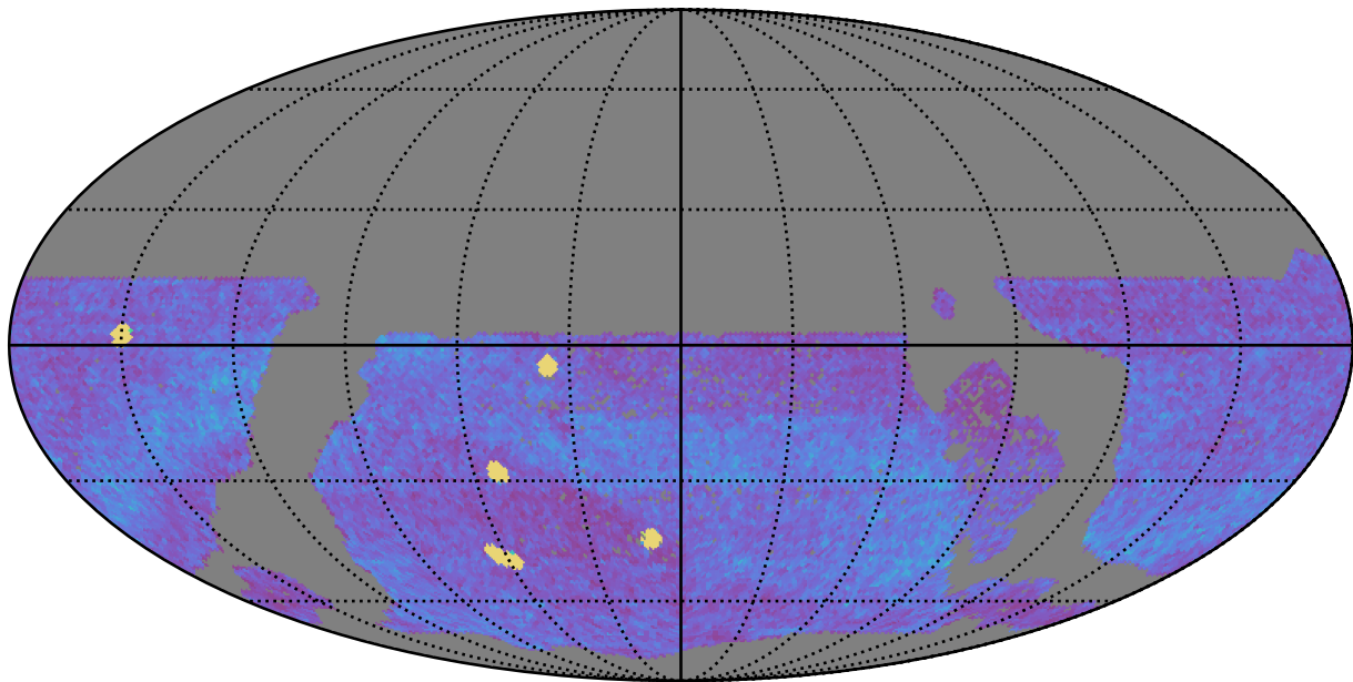
too_elab_r16_d2_giz_v3.4_10yrs WFD all bands: NVisits
