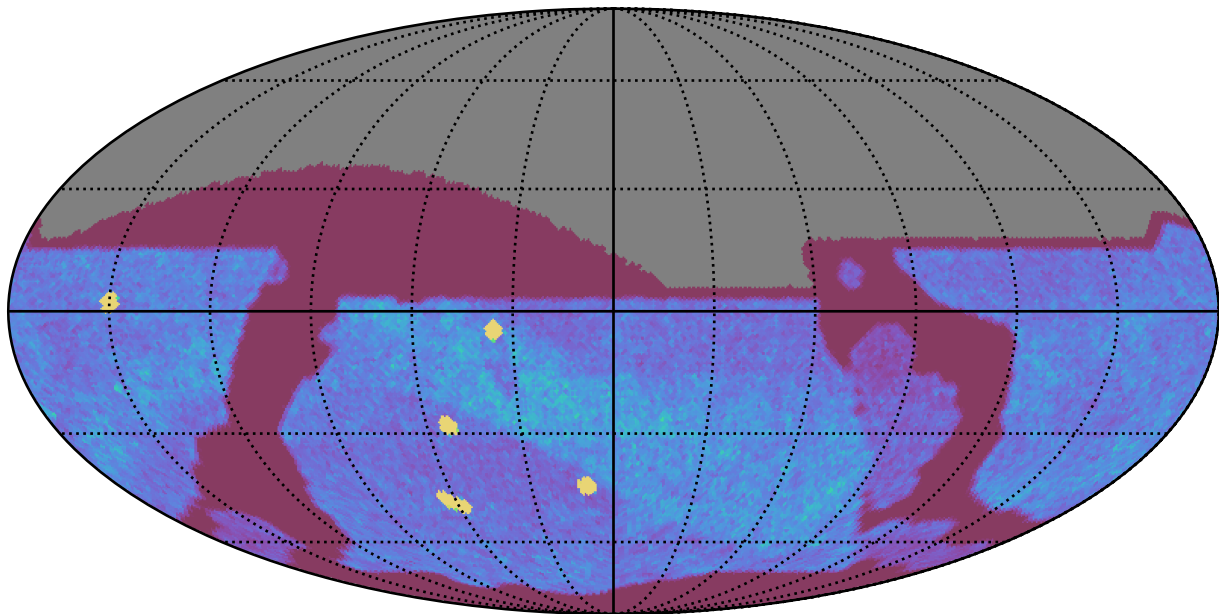
too_elab_r16_d2_giz_v3.4_10yrs All sky z band: NVisits
