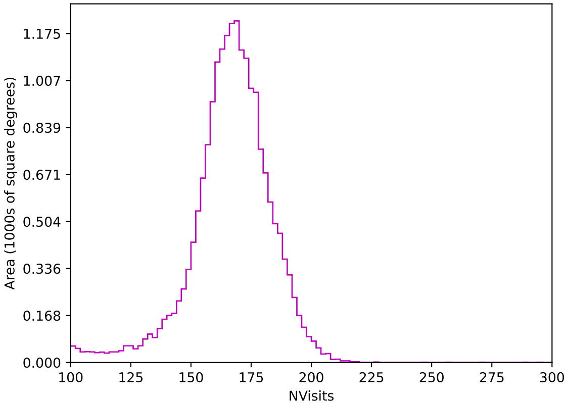
too_elab_r16_d2_giz_v3.4_10yrs All sky z band: NVisits
