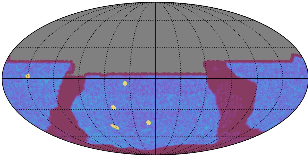
too_elab_r16_d2_giz_v3.4_10yrs All sky y band: NVisits
