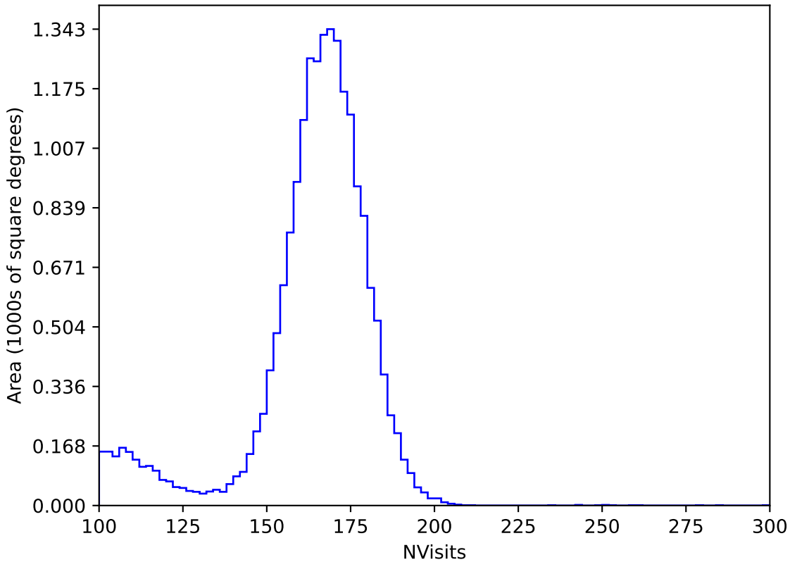
too_elab_r16_d2_giz_v3.4_10yrs All sky y band: NVisits
