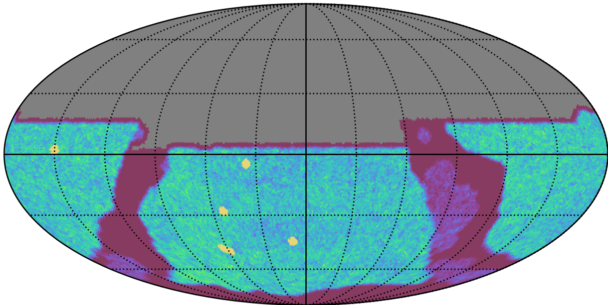
too_elab_r16_d2_giz_v3.4_10yrs All sky u band: NVisits
