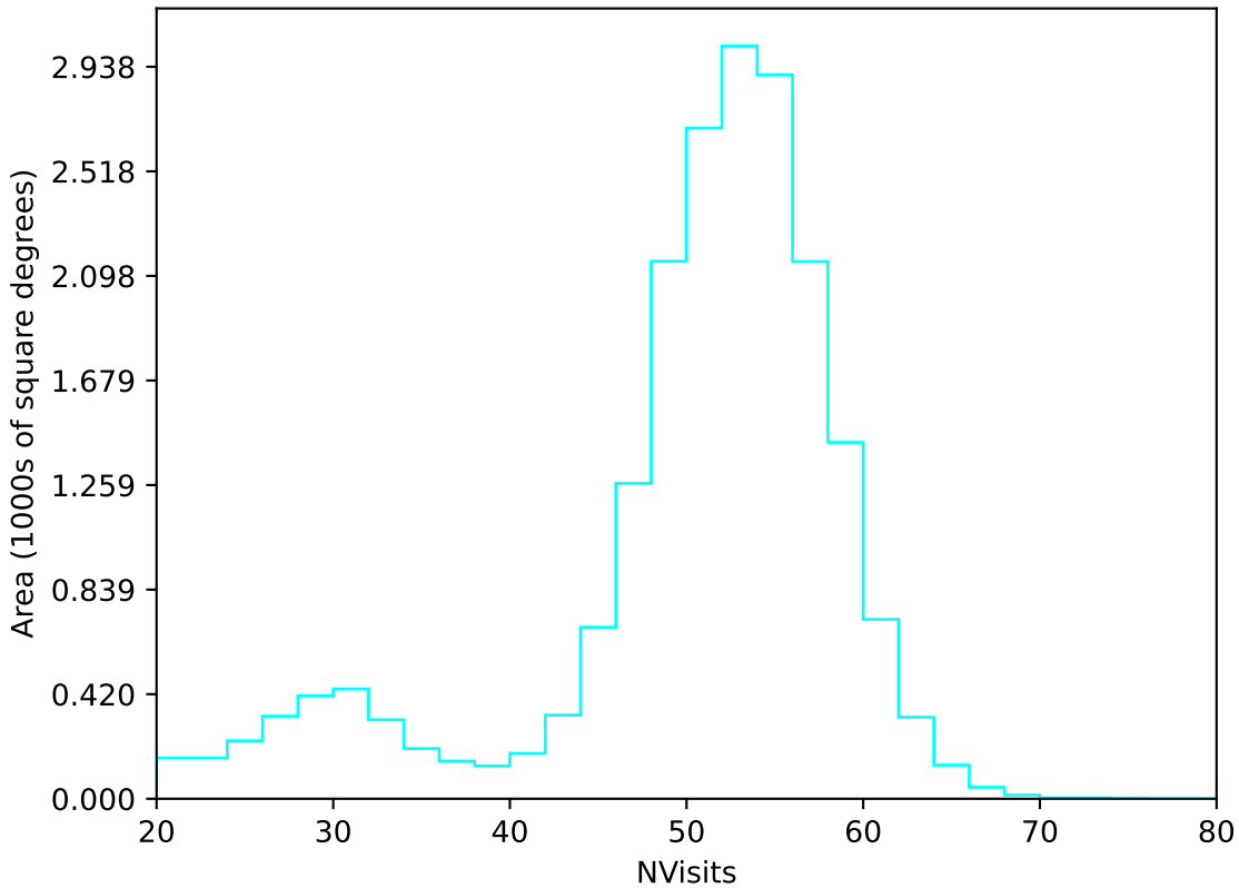
too_elab_r16_d2_giz_v3.4_10yrs All sky u band: NVisits
