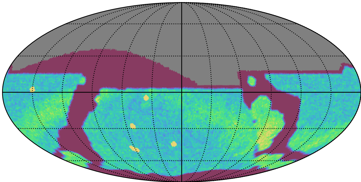
too_elab_r16_d2_giz_v3.4_10yrs All sky r band: NVisits
