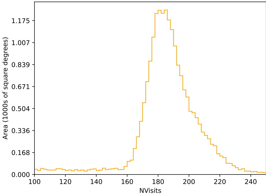
too_elab_r16_d2_giz_v3.4_10yrs All sky r band: NVisits
